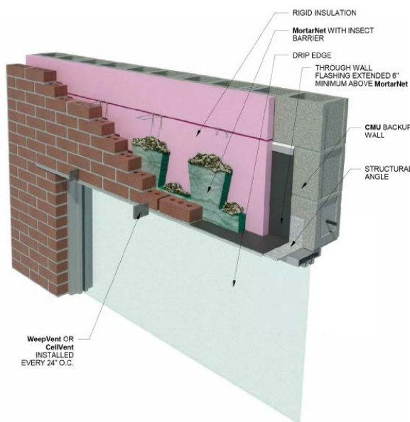
MortarNet with Insect Barrier Window Head Detail
