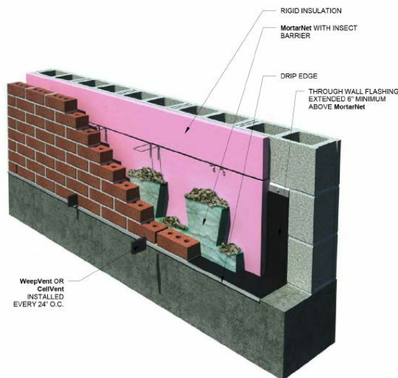
MortarNet with Insect Barrier Wall Base Detail
